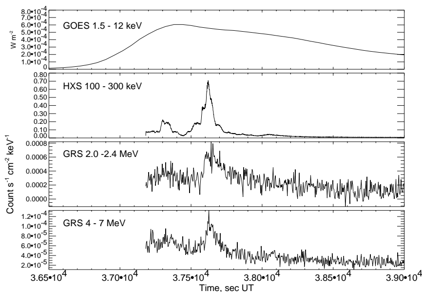
Figure 1. Time history of the 2000 July 14 flare observed by GOES and the Yohkoh WBS.
