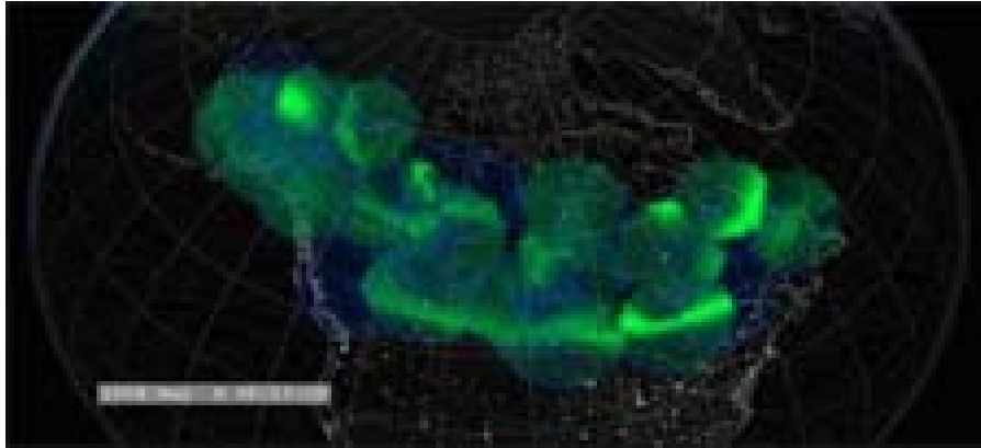
A collection of ground-based All-Sky Imagers (ASI) captures the aurora brightening caused by a substorm.
