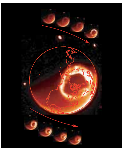
Evolution of the aurora during the July 15, 2000, Bastille Day magnetic storm. 1423UT–1512UT
