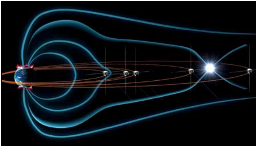
This illustration shows the THEMIS spacecraft within a depiction of the Earth's magnetic field. The release of magnetic energy is shown downstream, in the tail of the Earth's magnetosphere where the field lines intertwine and reconnect. The aurorae created in the ionosphere by the reconnection current are indicated above the Earth's polar regions.
