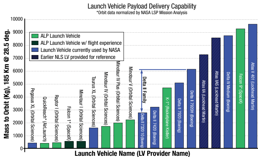
The Alternate Launch Vehicle Payload (ALP) delivery capability showing mass to 185 km orbit with a 28.5° inclination as a function of launch vehicle.
