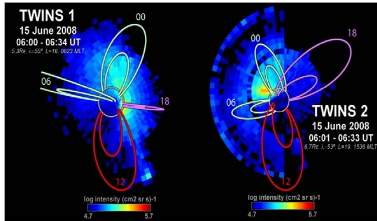
First-light stereo ENA image obtained by TWINS on 15 June 2008. The color indicates ENA flux. The Earth is in the center of each image, surrounded by dipole magnetic field lines at 4 and 8 Earth radii equatorial crossing-points. Field lines at noon (dusk) are colored red (lavender).
