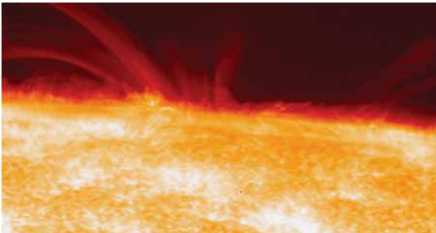
This picture was taken by Hinode's Solar Optical Telescope on November 11, 2006. In the foreground, this image reveals the fine-scale structure in the chromosphere that extends outward above the top of the convection cells, or granulation, of the visible solar surface layer, the photosphere. In the background, plasma above a sunspot traces out magnetic field lines into the corona.
