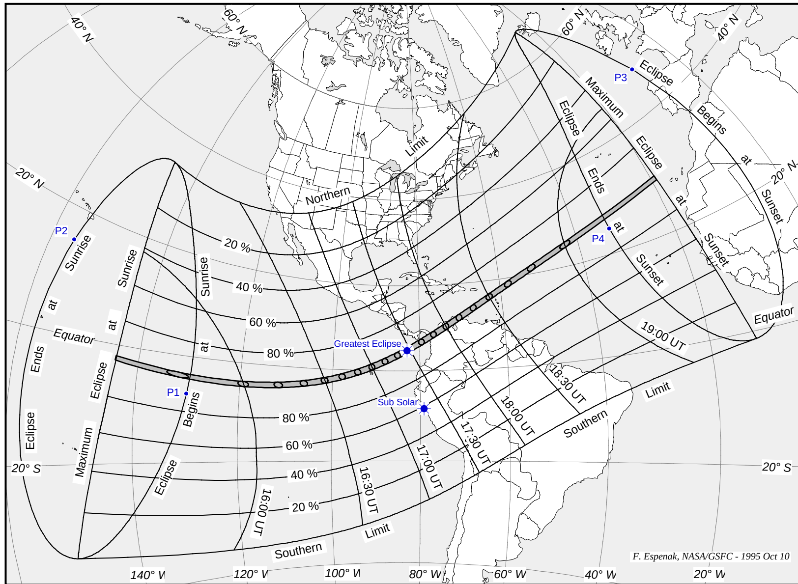
FIGURE 2: STEREOGRAPHIC PROJECTION MAP OF THE ECLIPSE PATH
