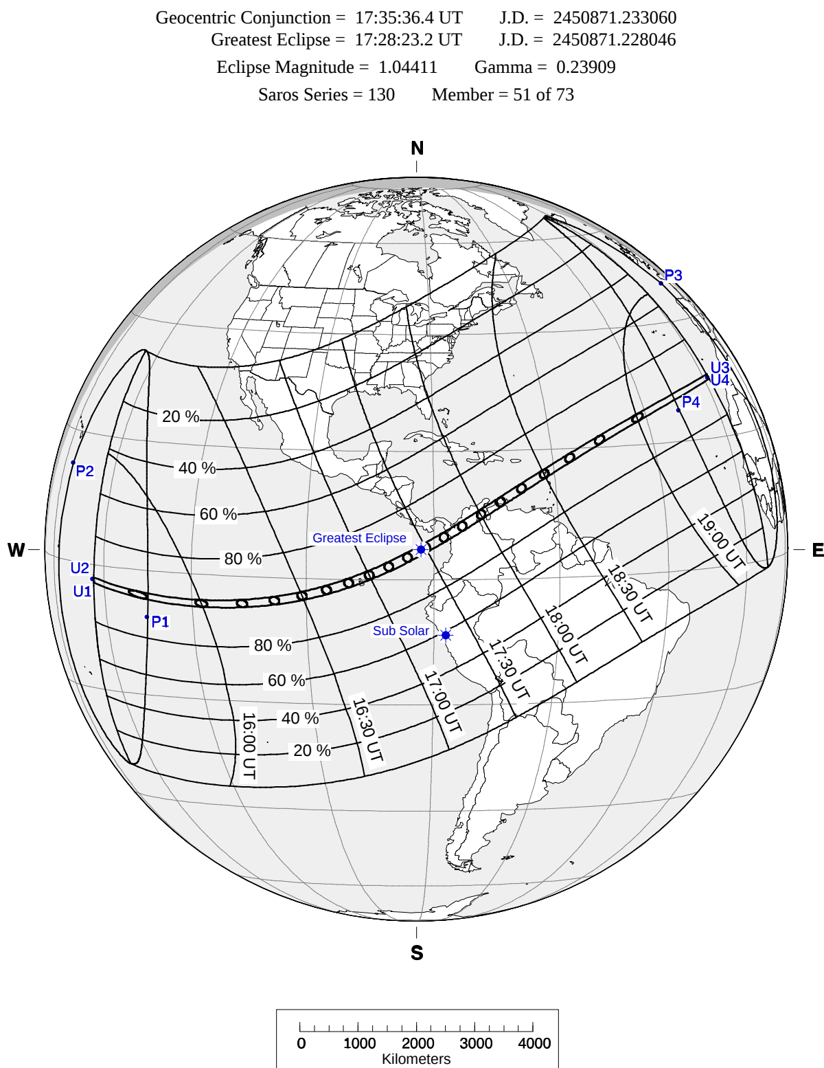
FIGURE 1: ORTHOGRAPHIC PROJECTION MAP OF THE ECLIPSE PATH
