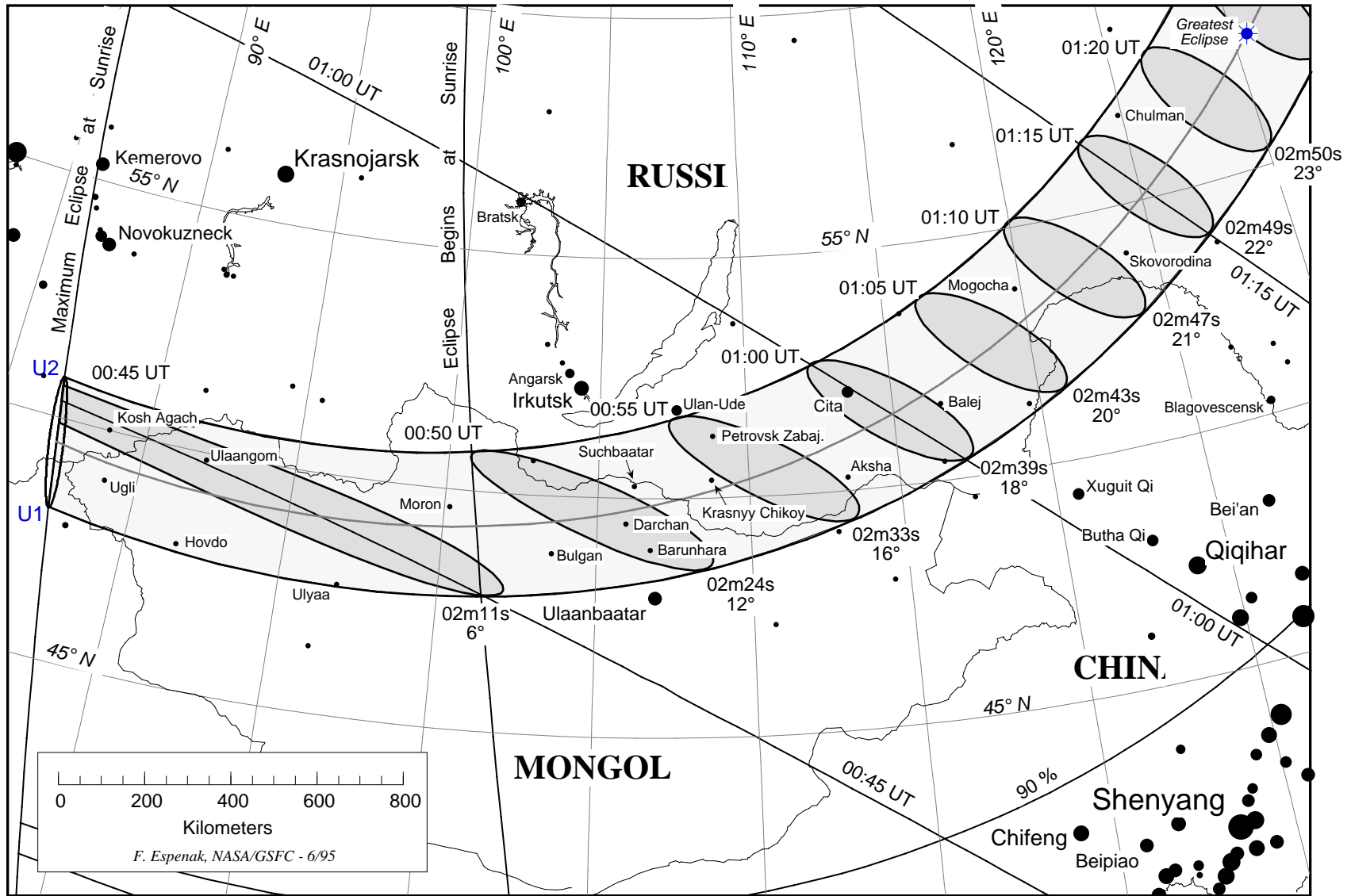
Figure 4: THE ECLIPSE PATH IN DE Total Solar Eclipse of 1997 Mar 9
