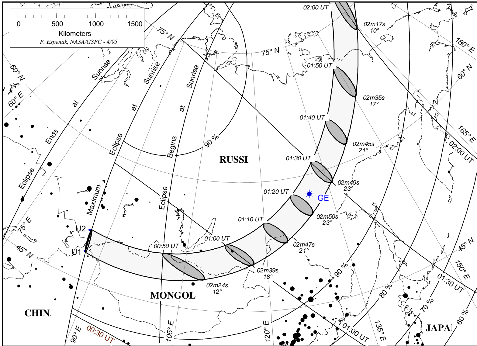
Figure 3: THE ECLIPSE PATH THROUGH Total Solar Eclipse of 1997 Mar 9
